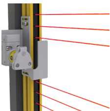
BRAVO for light curtains, mounted on the left BRV4A-1-1-CLSL-MPI
