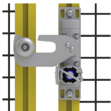
ALPHA for sliding doors, left-sliding ALP2S-1-1-CLSS-MP
